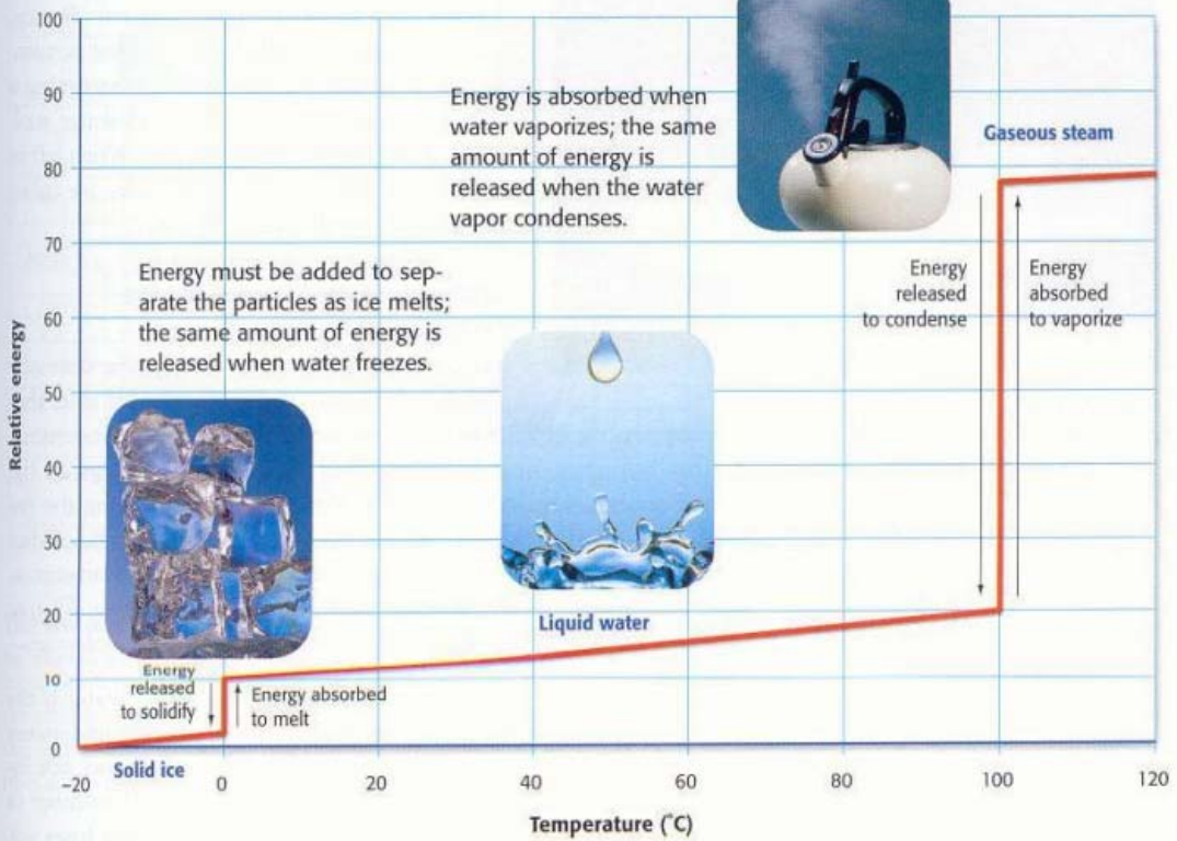
Figure 2-14 The Changes of State for Water
